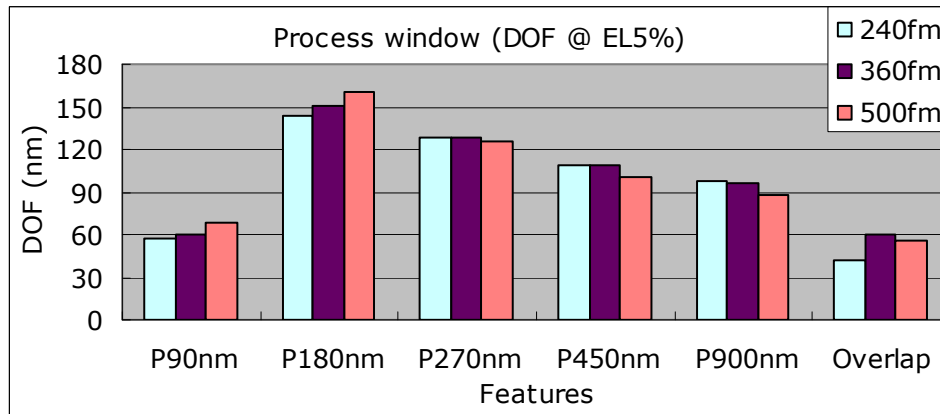
Fig.14 Summary of DOF @ EL5% (w/ SRAF)
