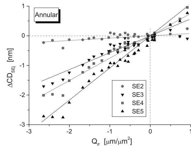
Fig. 12 \Delta CD - Q_F correlation for the two illumination modes of the experiment.
