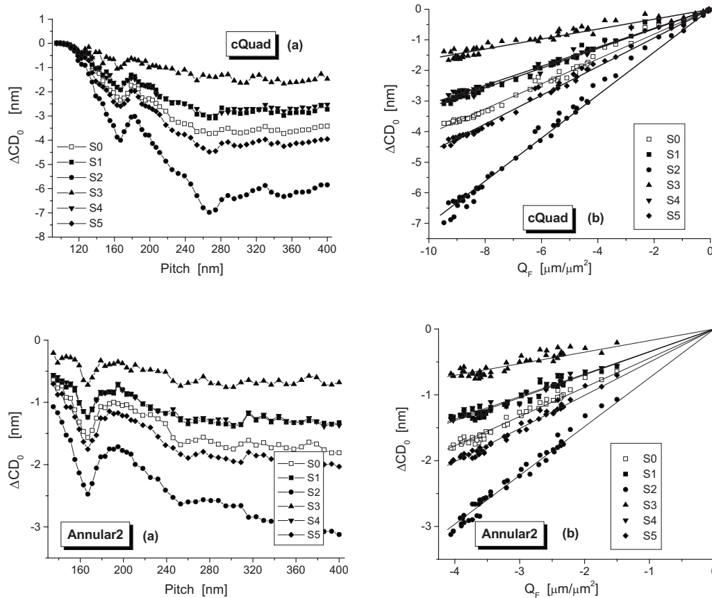
Fig. 6 Calculated values of finite-bandwidth–monochromatic CD differences, \Delta\text{CD}_0(P) , for the six laser spectra of this study, plotted versus pitch as well as versus Q_F(P) . Examples for the cQuad and one of the Annular2 settings of Table 3, calculated with the FRM.
