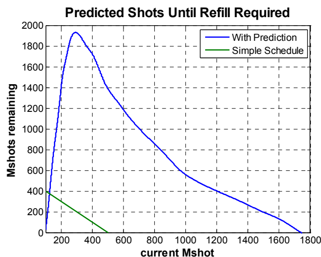
Figure 9: Prediction of remaining shots in a gas life, comparison using advanced prediction and simple schedule.
