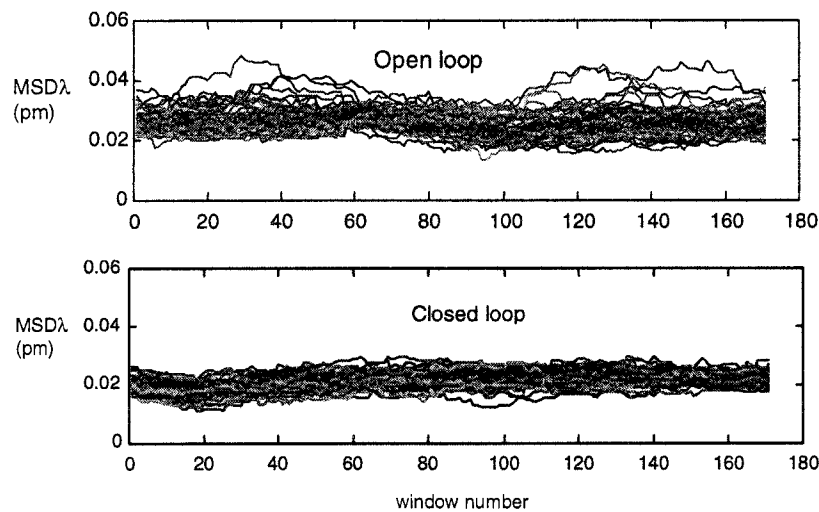
Figure 12: Open and closed loop (active damping) MSD\lambda data at 2100 Hz repetition rate.
