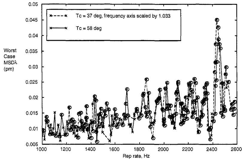
Figure 2: Worst-case burst-mode MSD\lambda as a function of repetition rate, with all wavelength control disabled, and all random components averaged out in post-processing: comparing two chamber temperatures.
