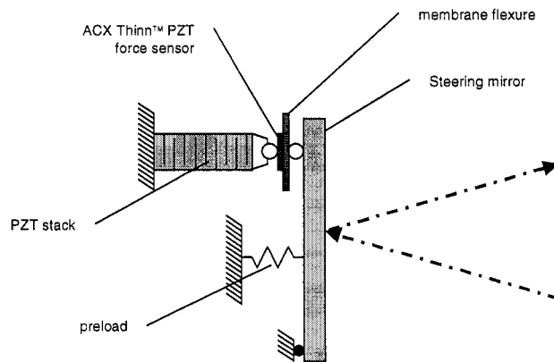
Figure 9: Mechanical arrangement of actuator, sensor, and steering mirror used in active damping loop.
