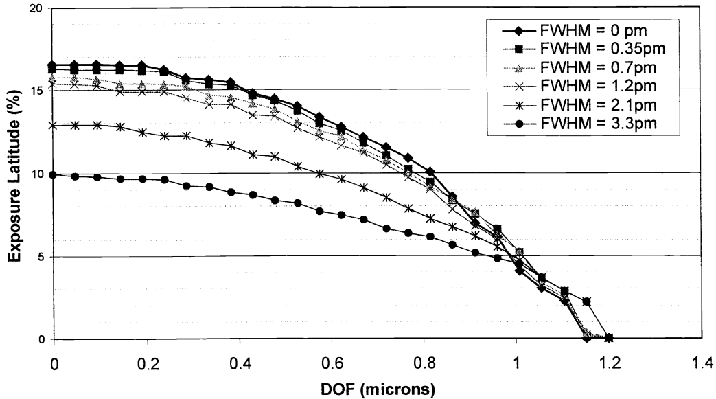
Figure 5. Sensitivity of the focus-exposure process window to laser bandwidth. Numerical aperture of the lens is set at 0.6 and partial coherence factor \sigma at 0.75.
