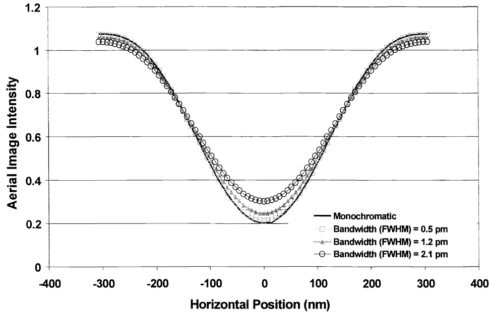
Figure 3. Degradation of the aerial image of a 180 nm line (500 nm pitch) with increasing laser bandwidth for a chromatic aberration response of 0.225 \mu\text{m}/\text{pm} .
