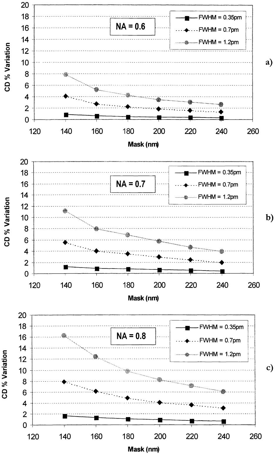
Figure 4. Impact of laser bandwidth on aerial image CD variations (%) of isolated lines with respect to the monochromatic illumination for different lens NAs: a) NA = 0.6 ; b) NA = 0.7 ; and c) NA = 0.8 .
