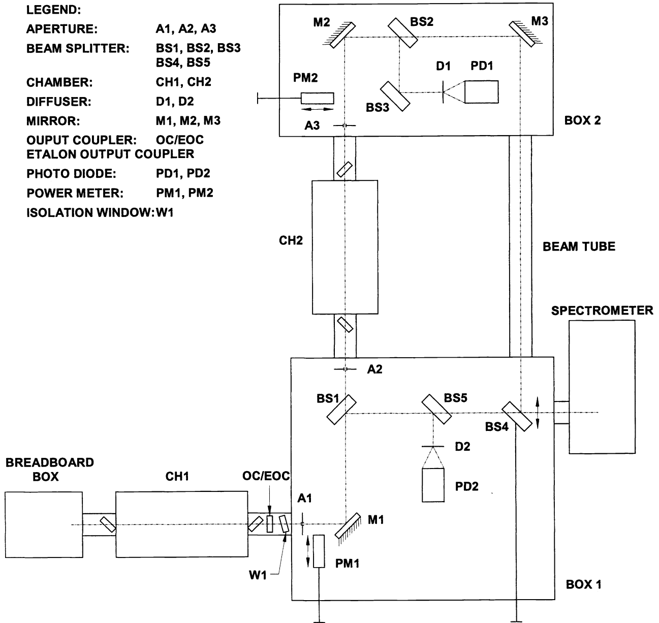
Figure 1: Experimental setup
