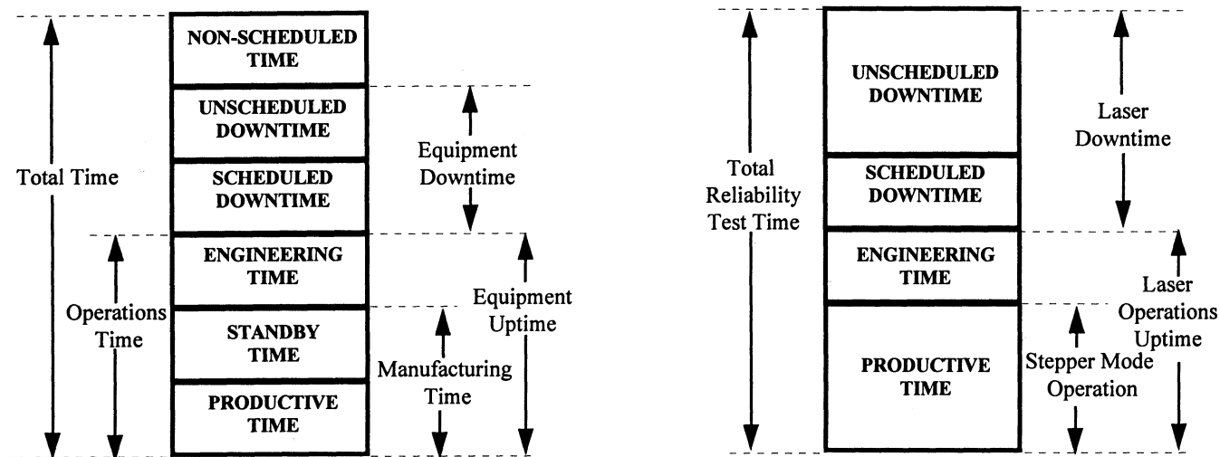
ELS-5000 States During Reliability Test
