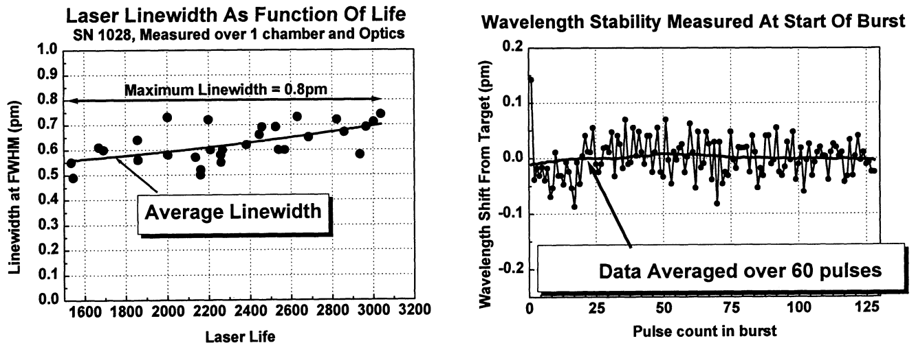
Figure 6. Spectral Data measured on the laser.
